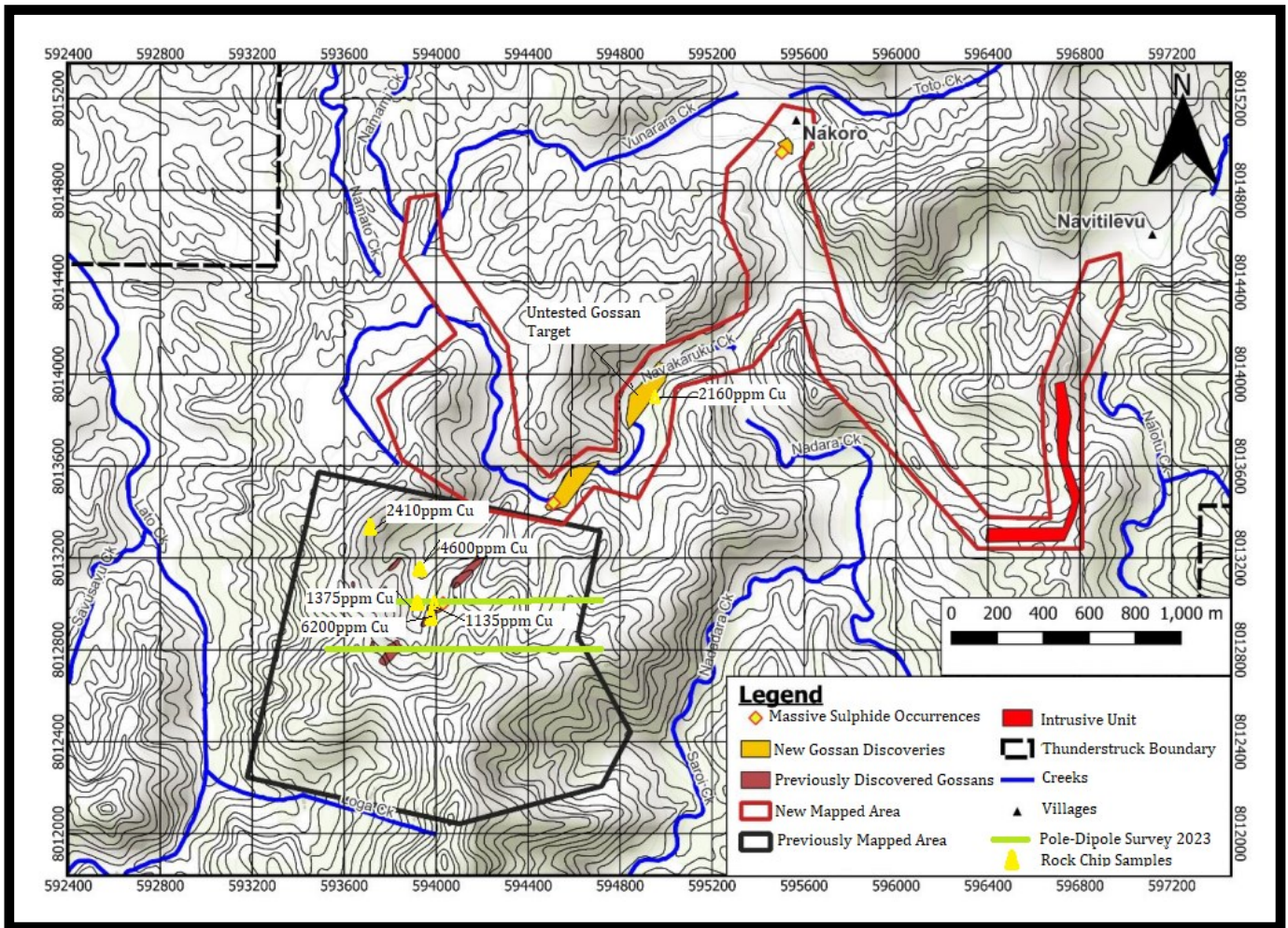
Figure 2: Map of Nakoro showing newly mapped area and some points of Interest.
