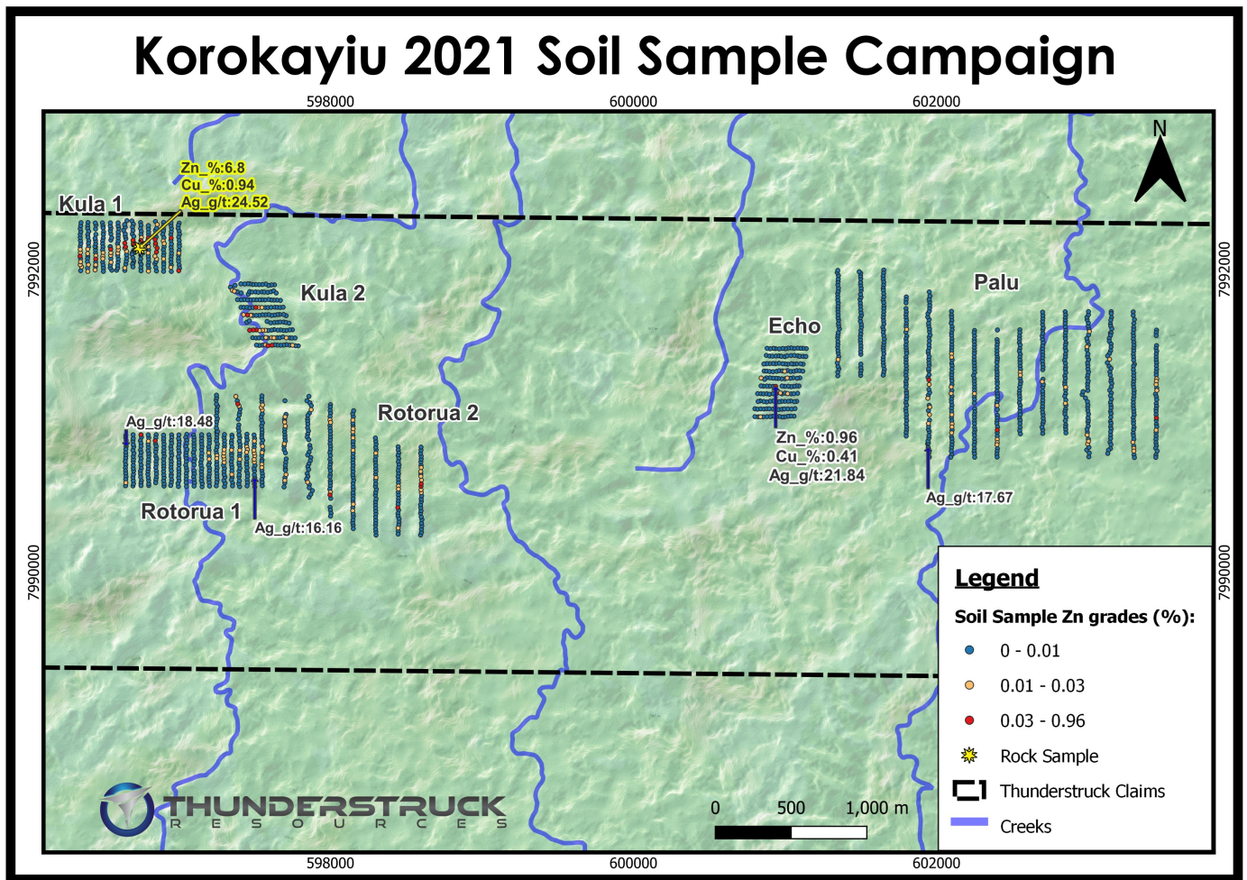
Figure 4: 2021 Korokayiu zinc (Zn) soil sampling results
